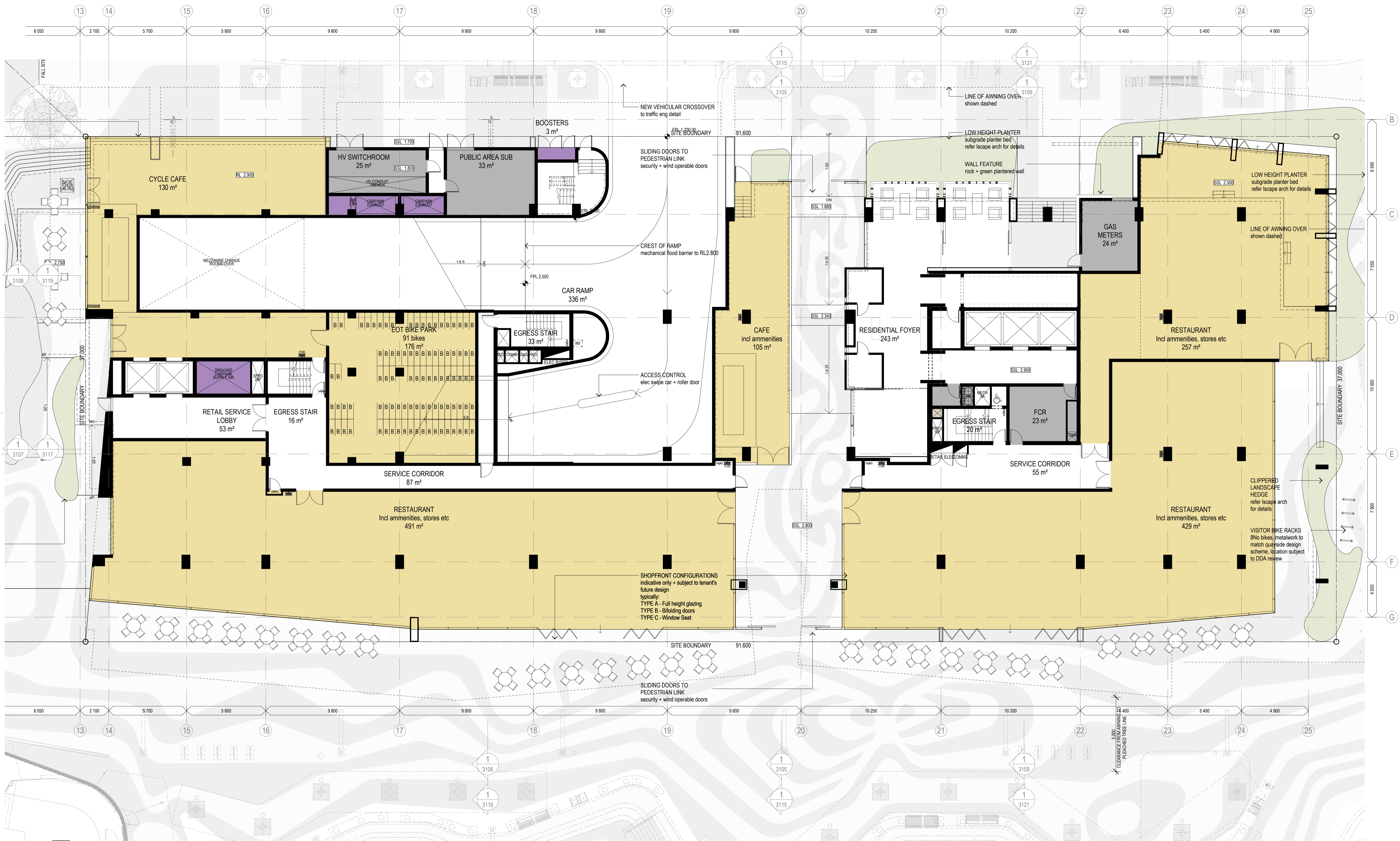
1 LOT 10 FLOOR PLAN - GROUND SCALE 1:125 @ A1 SCALE 1:250 @ A3
